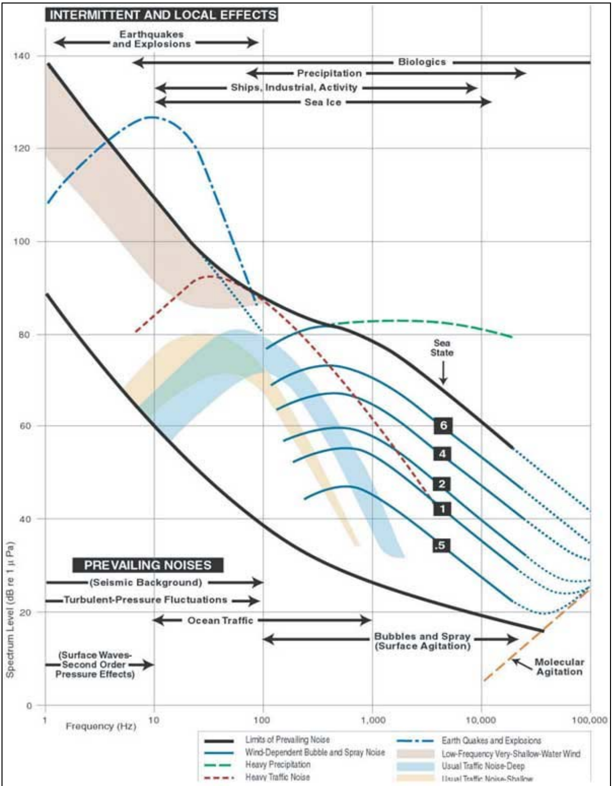
Figure D-3: Oceanic Ambient Noise Levels from 1 Hertz to 100,000 Hertz, Including Frequency Ranges for Prevalent Noise Sources
