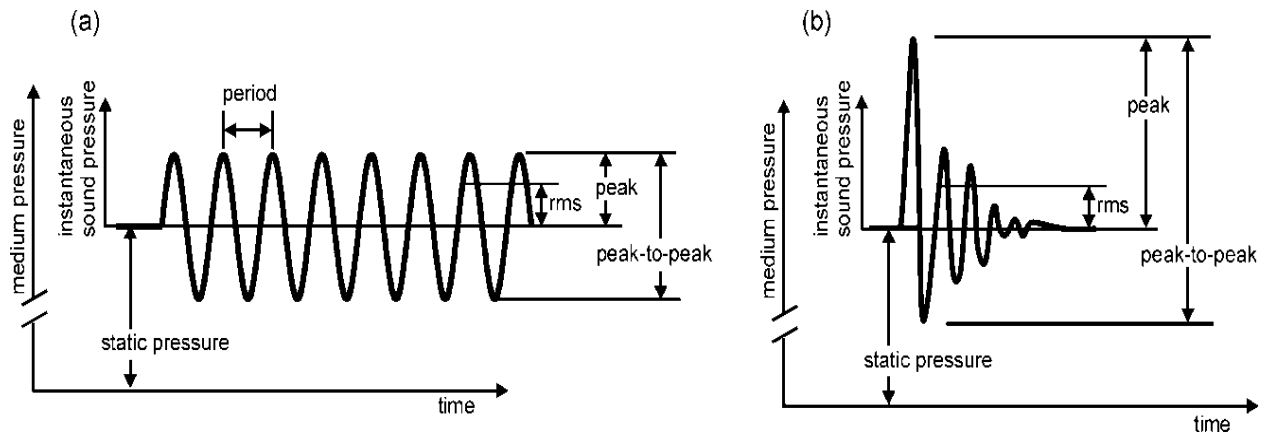
Figure D-5: Various Sound Pressure Metrics for a Hypothetical (a) Pure Tone (Non-Impulse) and (b) Impulse Sound
