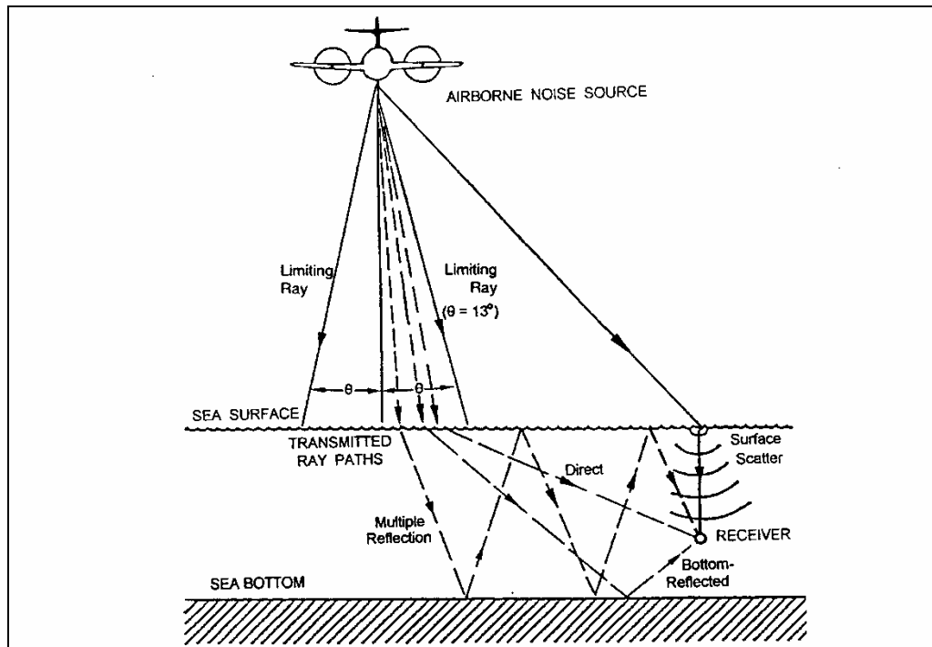
Figure D-2: Characteristics of Sound Transmission through the Air-Water Interface
