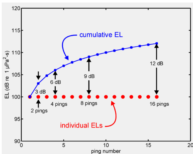
Figure D-6: Summation of Acoustic Energy (Cumulative Exposure Level, or Sound Exposure Level) from a Hypothetical, Intermittently Pinging, Stationary Sound Source
