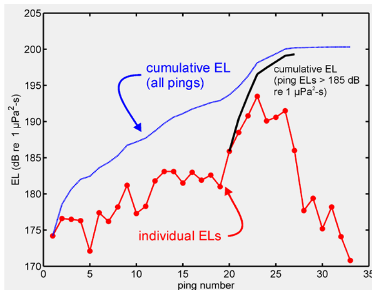
Figure D-7: Cumulative Sound Exposure Level under Realistic Conditions with a Moving, Intermittently Pinging Sound Source (Cumulative Exposure Level = Sound Exposure Level)
